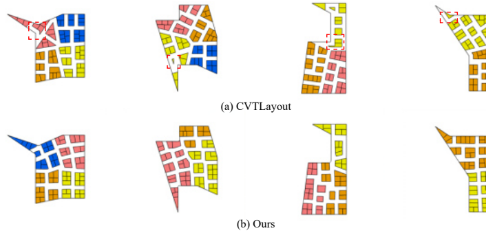
Fig. 8. Comparison between our diffusion-based method and CVTLayout.
