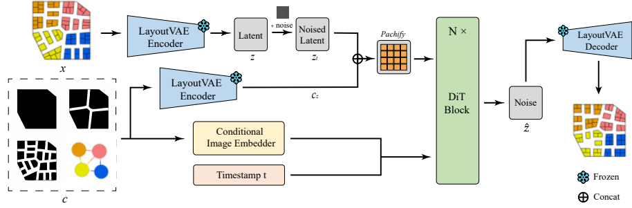
Fig. 3. The pipeline of our diffusion-based generative model. The layout image and the conditional image are taken as inputs. The layout image is first encoded into the latent space by the encoder and then noised. For the conditional image, on one hand, its features are extracted by an image encoder, combined with the timestamp, and fed into the DiT-block; on the other hand, it is also encoded into the latent space by the encoder to align with the layout image’s latent space. Subsequently, the conditional image’s latent features are concatenated with the noisy layout latent features along the channel dimension. Following DiT [27], we divide images into 16 \times 16 patches, embed them as tokens, and input them into the Transformer. Then, they are fed into the DiT-block, and finally, the output of the model is reconstructed into a floorplan.
